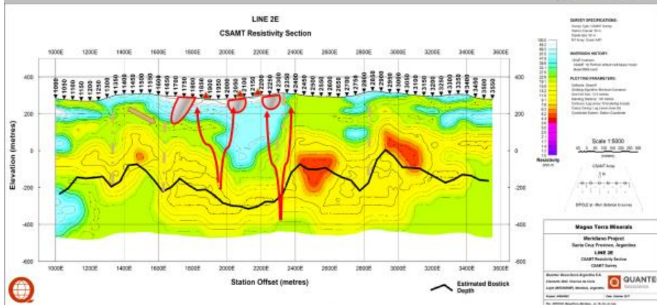
FIGURE 2, CSAMT LINE 2, THE CENTRAL LINE OF THREE TRAVERSING THE EL MERIDIANO PROJECT.
