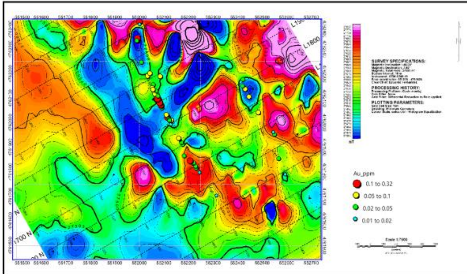
FIGURE 3, GERTRUDIS GROUND MAGNETIC, REDUCED TO THE POLE, WITH SURFACE GOLD
