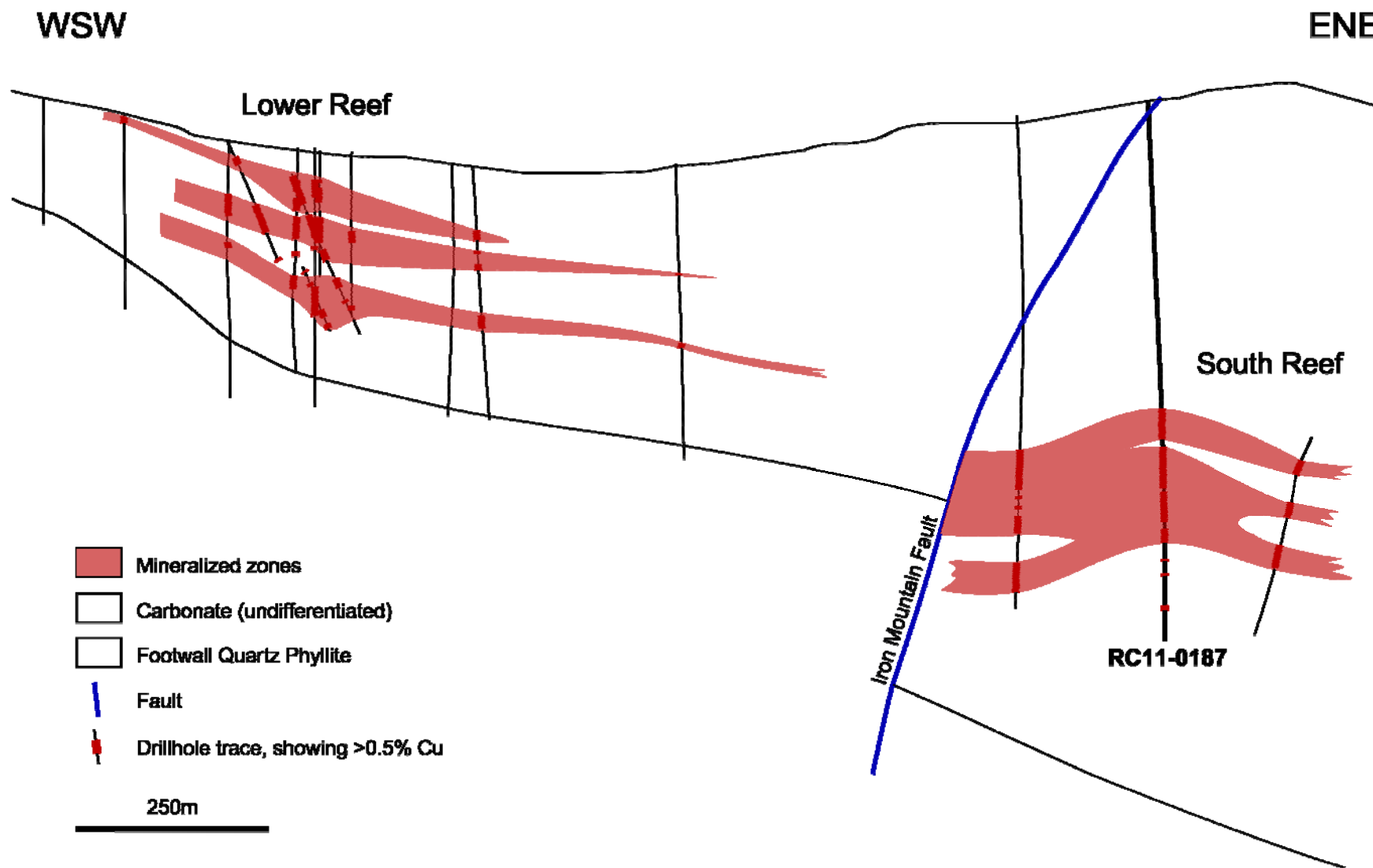
Figure 2: Bornite Cross Section Map
