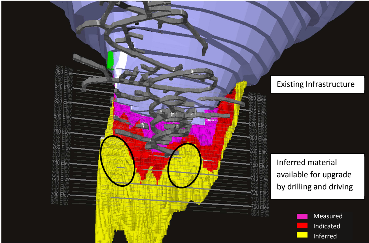
Figure 1. Isometric view showing remaining Dikulushi Mineral Resources below the Open Pit, looking southwest
