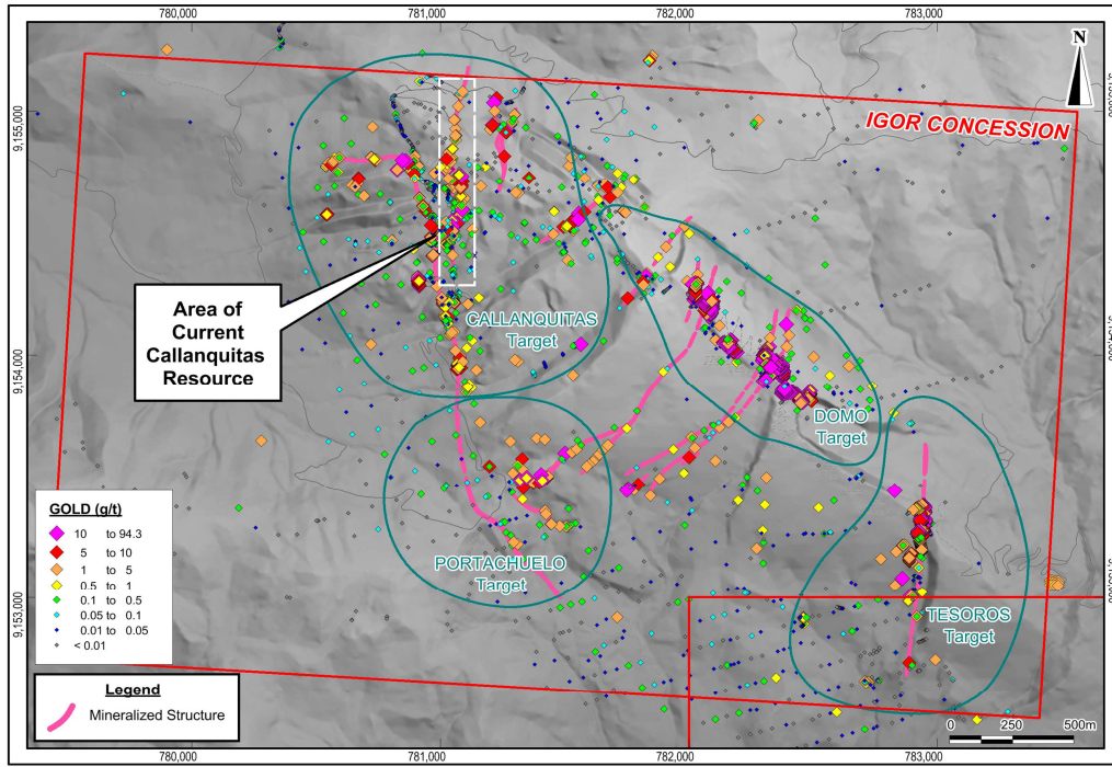
Figure 2 - Gold in surface samples, mineralized structures and target areas.
