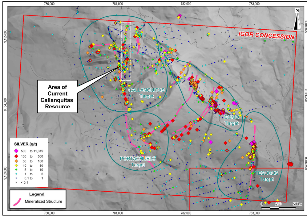
Figure 3 - Silver in surface samples, mineralized structures and target areas.
