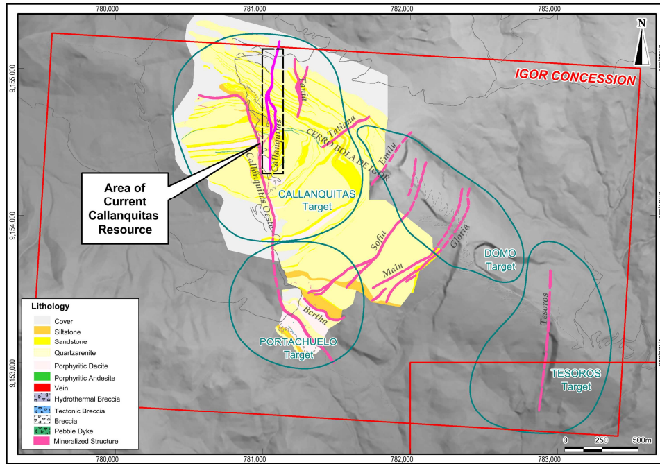
Figure 1 - 1:1,000 scale mapping on the Igor Property
