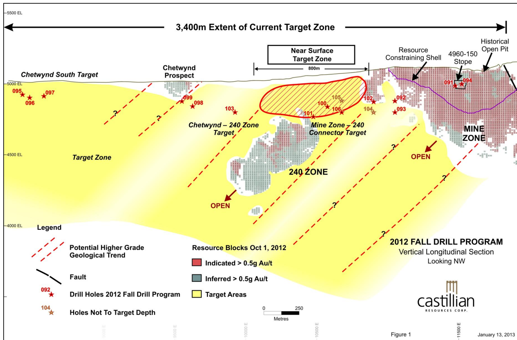
FIGURE 1: HOPE BROOK LONGITUNDINAL SECTION WITH TARGETS AND DRILL HOLES COMPLETED.
