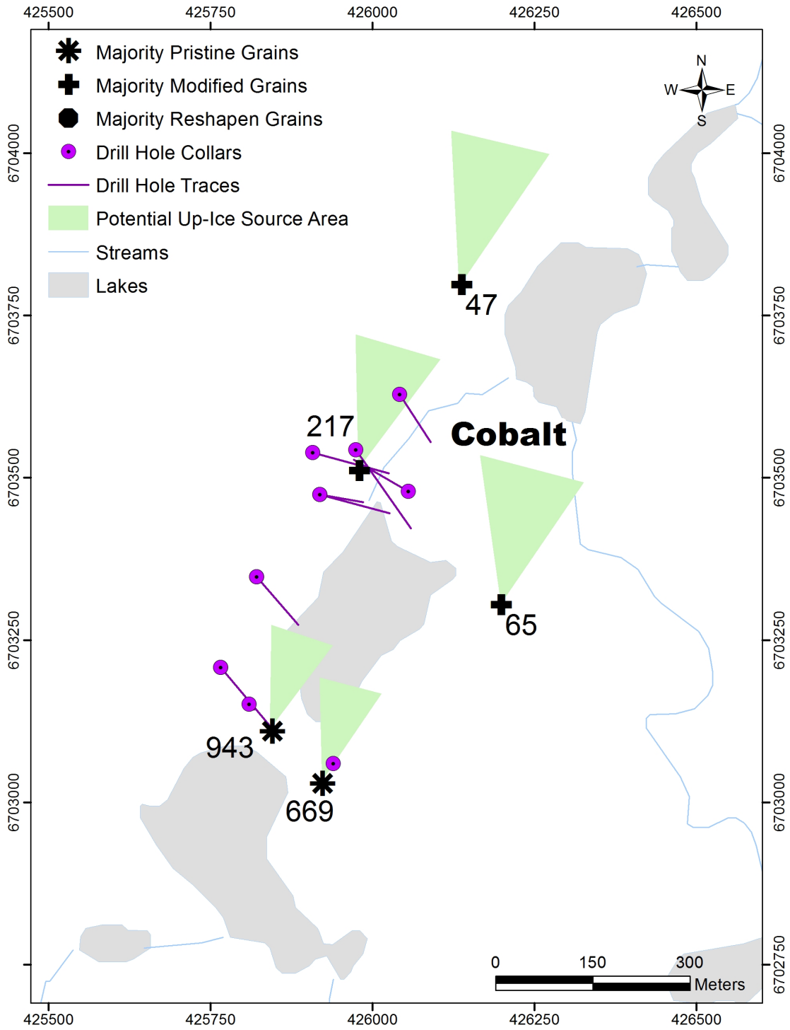
Figure 2. Gold grains from bulk till samples at Cobalt discovery
