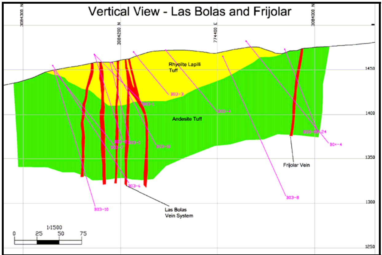
Interpreted geological cross section of the Las Bolas and Frijolar Veins looking north east. (The Las Bolas- Los Hilos Property Technical Report by Victor Jaramillo Page 21)
