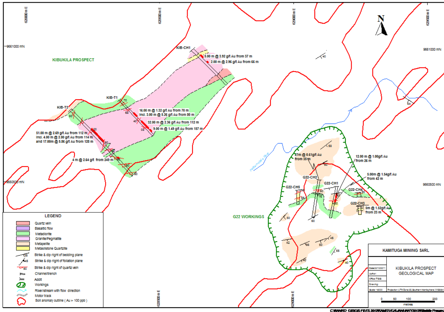
Figure 3: Geological map of the Kibukila and G22 Prospects showing soil anomalies (Au > 100 ppb) and trench results.
