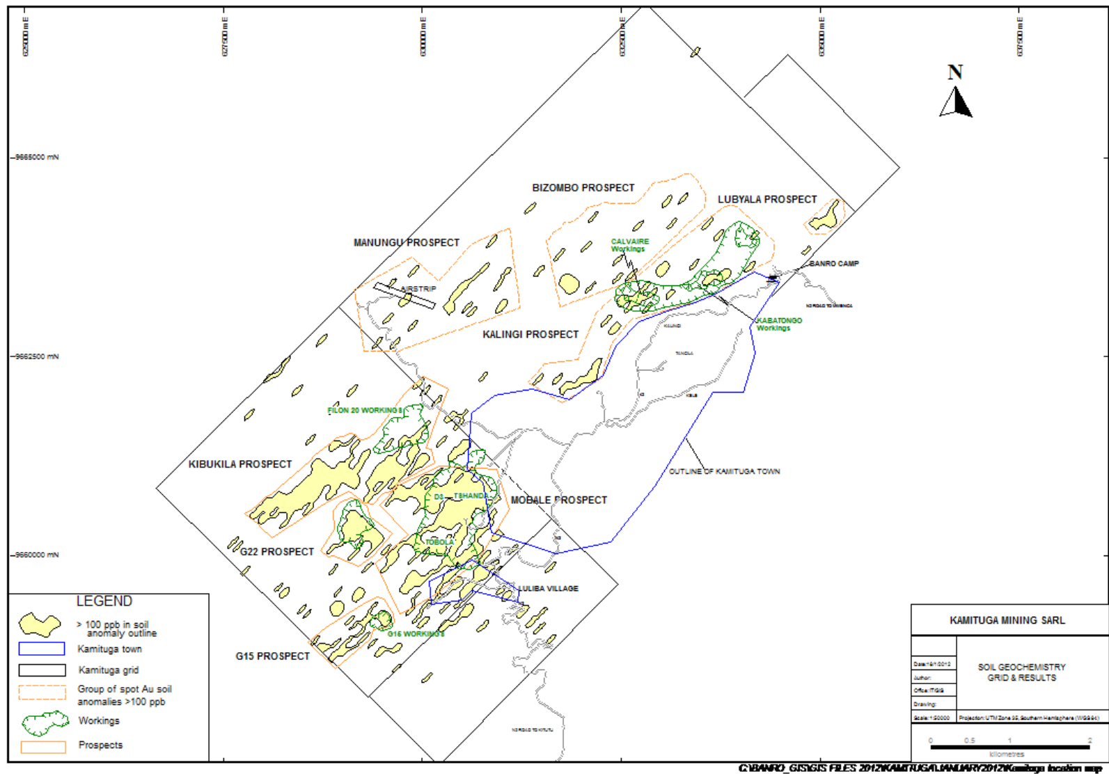
Figure 1: Location map of the Central Kamituga soil grid showing old workings, soil anomalies (Au > 100 ppb) and prospects.
