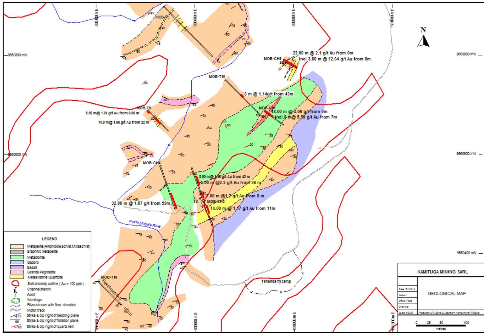
Figure 2: Geological map of the Mobale Prospect showing trench results and soil anomalies (Au > 100 ppb).
