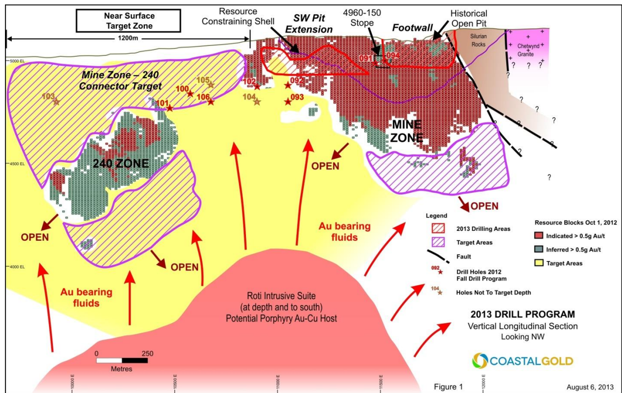
FIGURE 1: 2013 DRILL PROGRAM LONGITUDINAL SECTION
