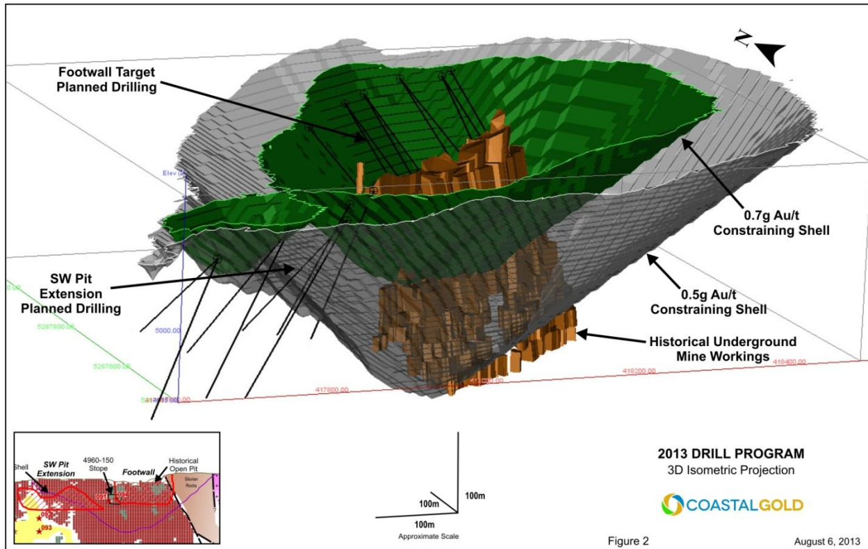
FIGURE 2: 2013 DRILL PROGRAM 3-D ISOMETRIC PROJECTION
