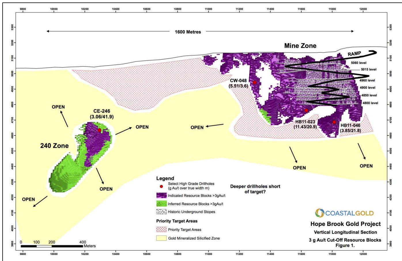
FIGURE 1: VERTICAL LONGITUDINAL SECTION SHOWING DISTRIBUTION OF RESOURCE BLOCKS IN THE MINE ZONE AND 240 ZONE, HOPE BROOK GOLD PROJECT
