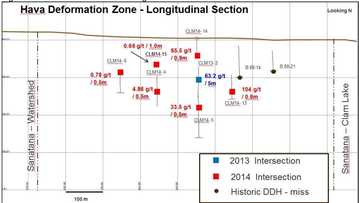
Figure 2: Hava Deformation Zone Longitudinal Section.
