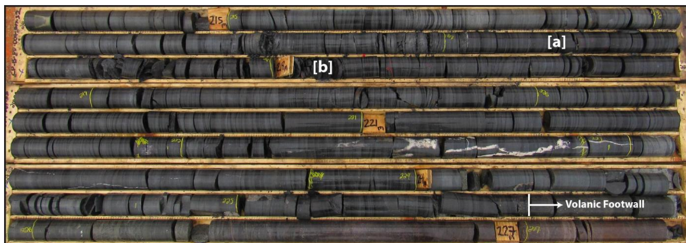
Figure 2. Disseminated bornite (copper sulphide) within the basal Rae Group of drill hole CP15_DD009; boxes shown are from 214.60 to 227.32 metres.
