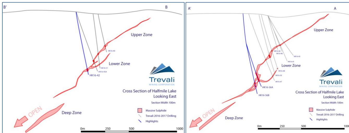
Figure 2: Cross sections of the Halfmile deposit showing 2016-2017 drill hole data.
