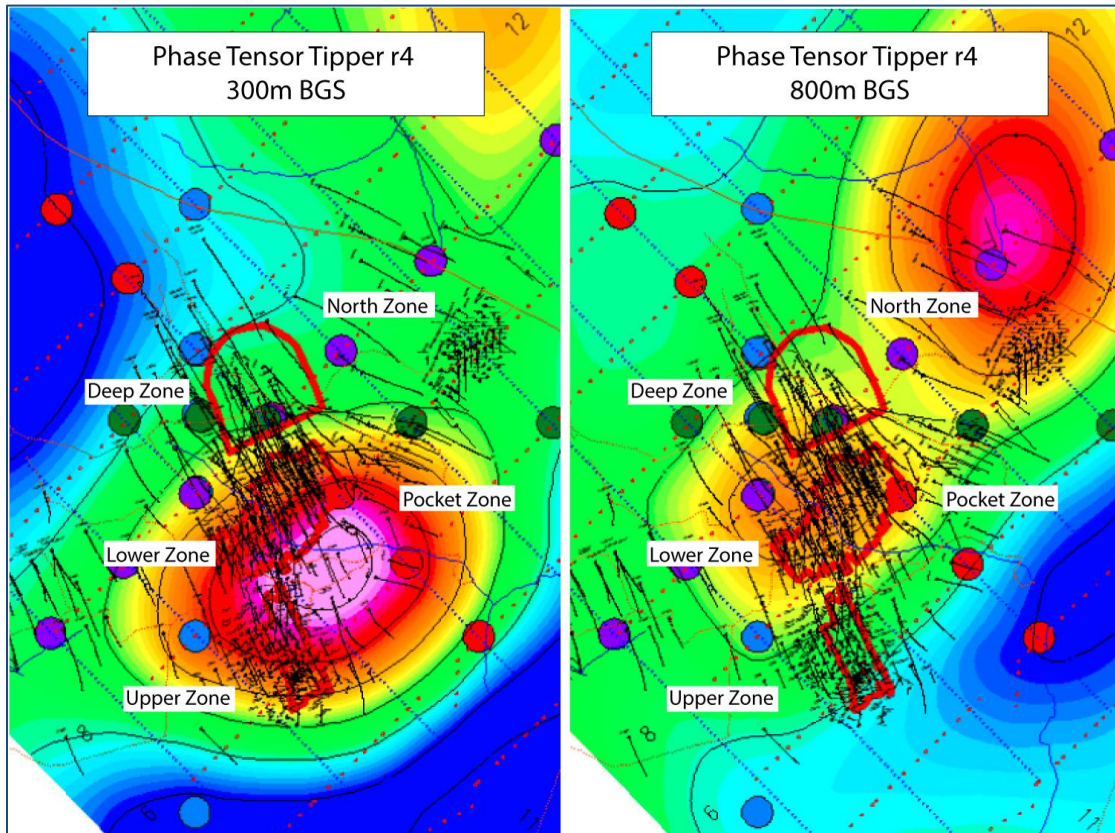
Figure 4: Halfmile Deposit AMT survey showing outline of mineralization and resistivity lows at different depths. Colored dots represent measurement stations.
