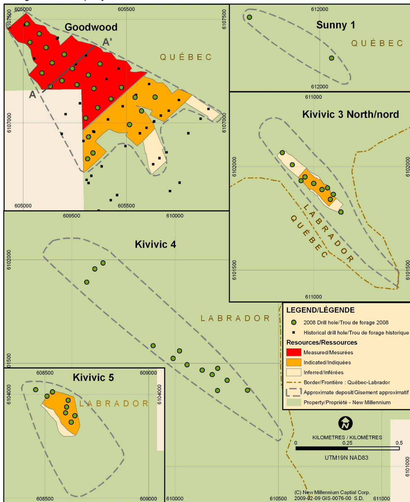
Figure 2b – Property Detail – DSO 4
