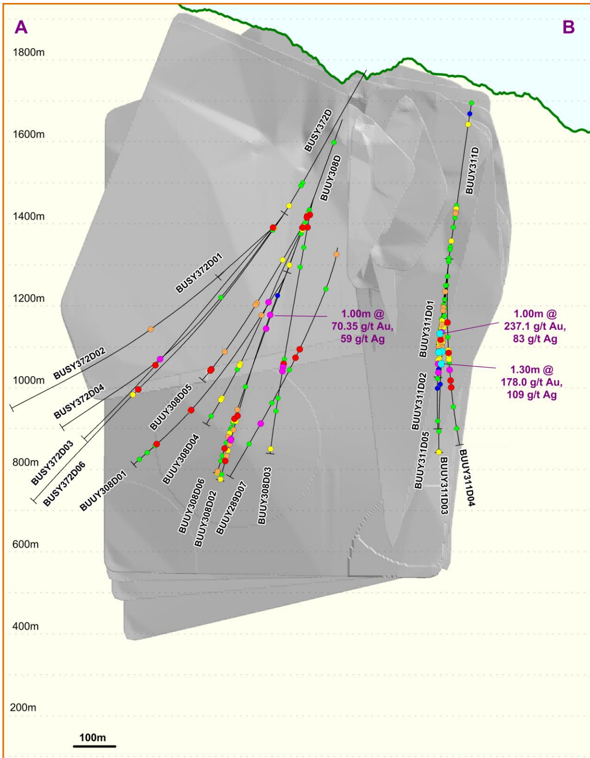
Figure 2 – Long section (Line A-B on Figure 1) showing highlights of new drilling against the 2014 Veta Sur mineral resource envelope.
