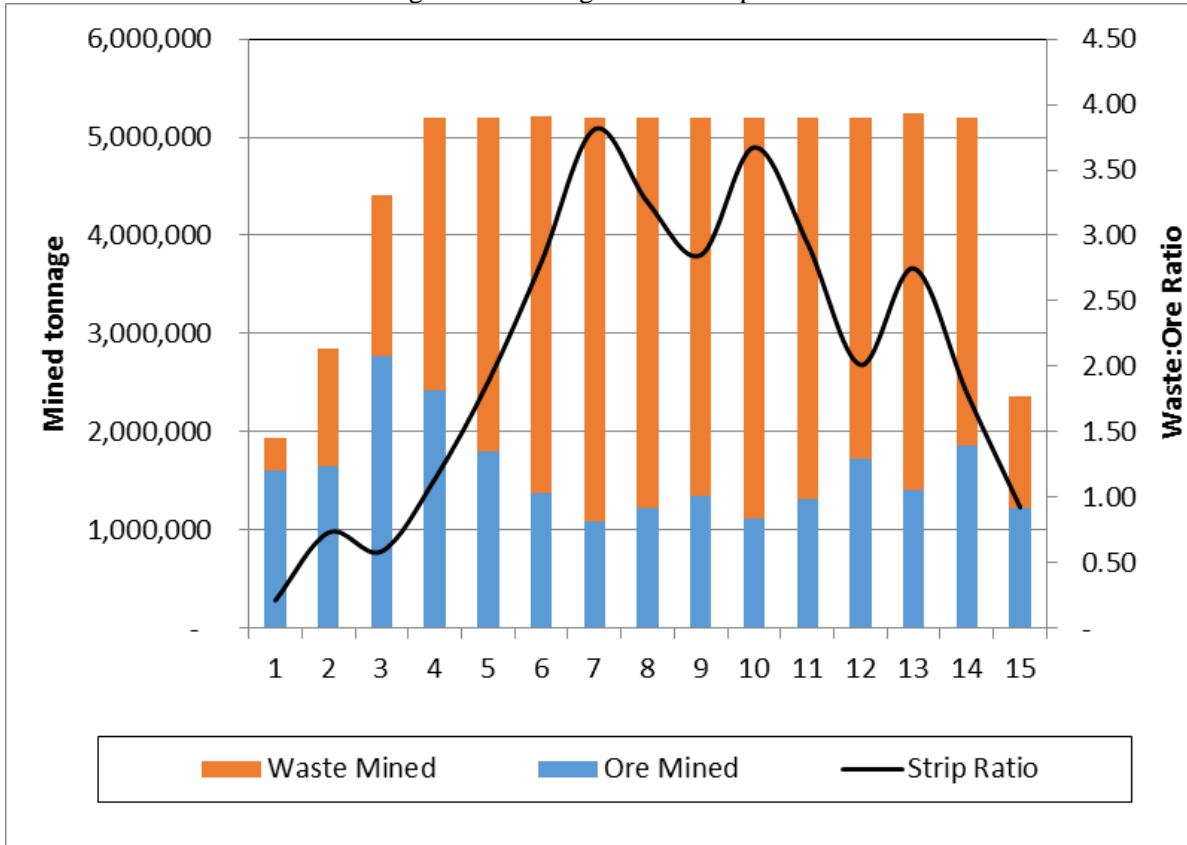
Figure 2 - Mining rate and strip ratio
