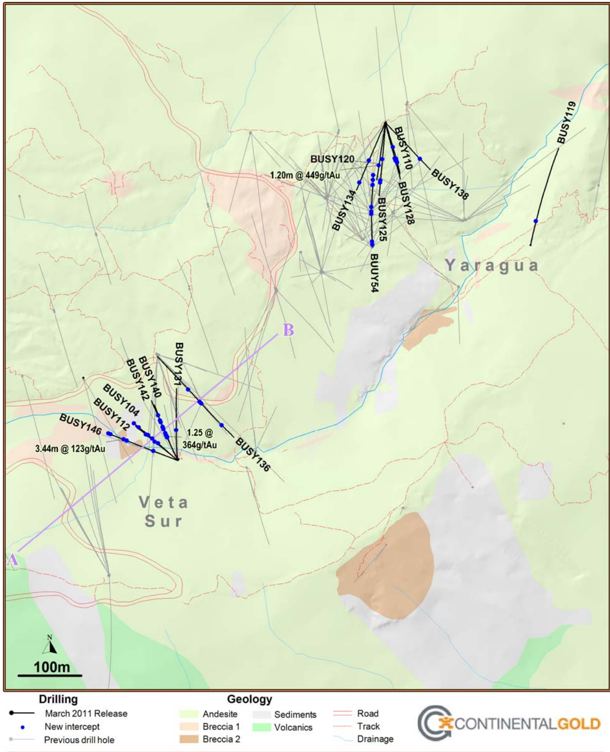
Figure 2 – Plan View of New Drilling
