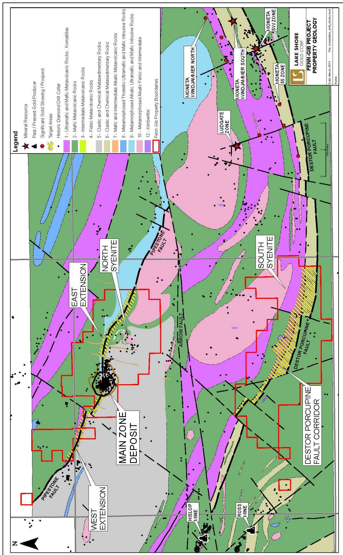
Figure 2. Property Geology
