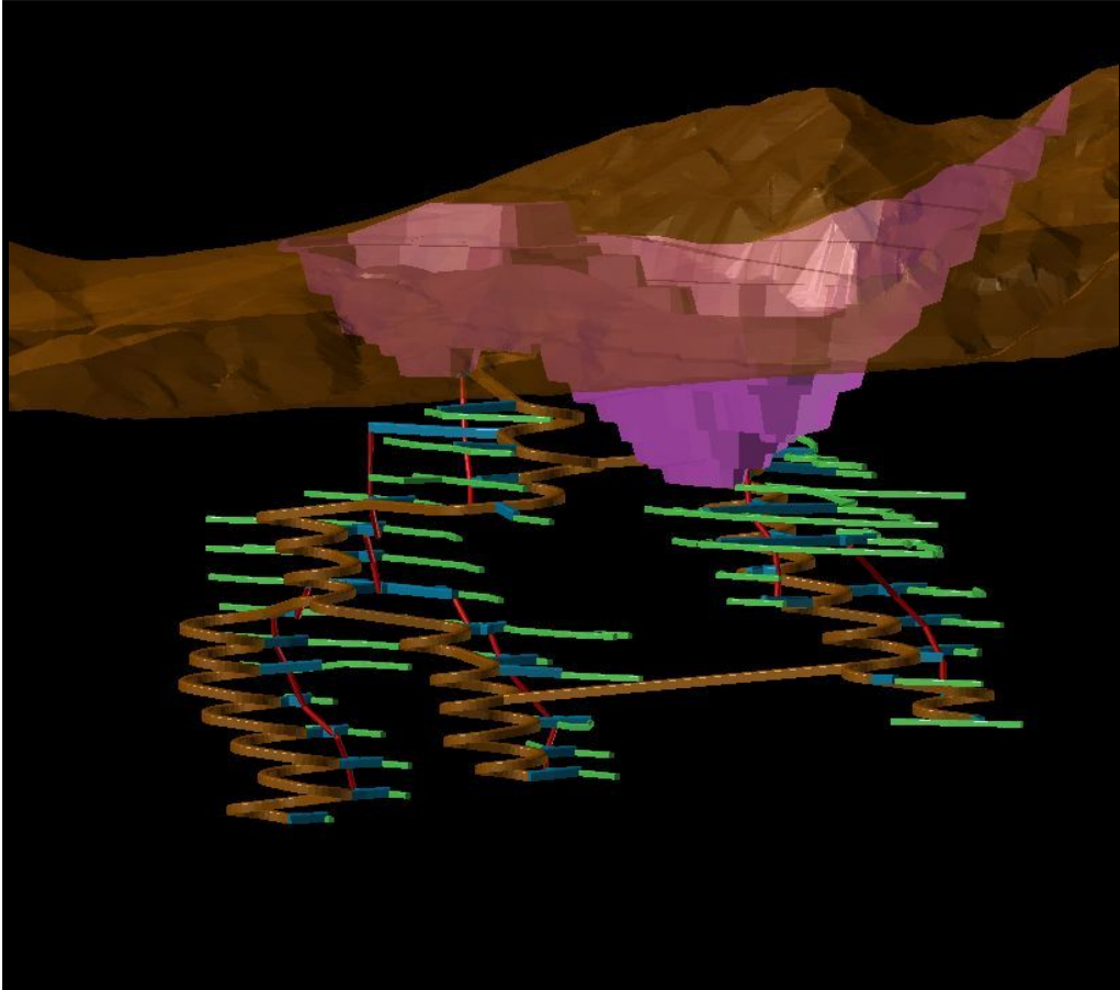
Casoso Proposed Open Pit and Underground Development looking south.
