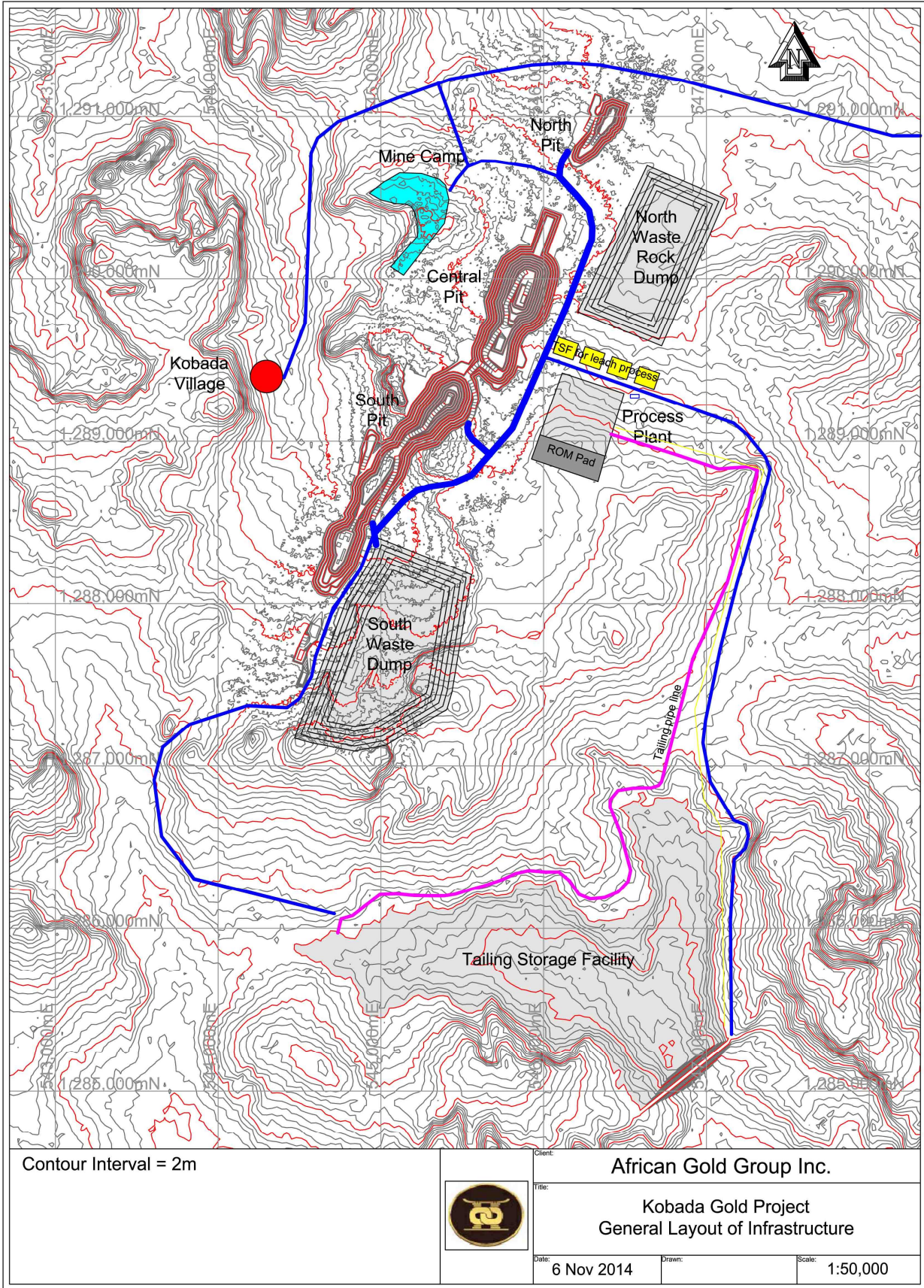
Figure 3 – General Site Layout
