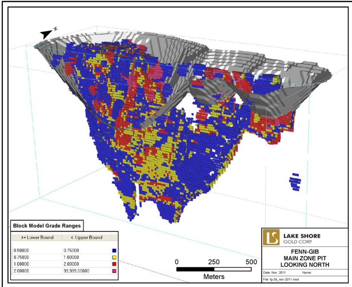
Figure 1. 3D View of Whittle Pit Shell
