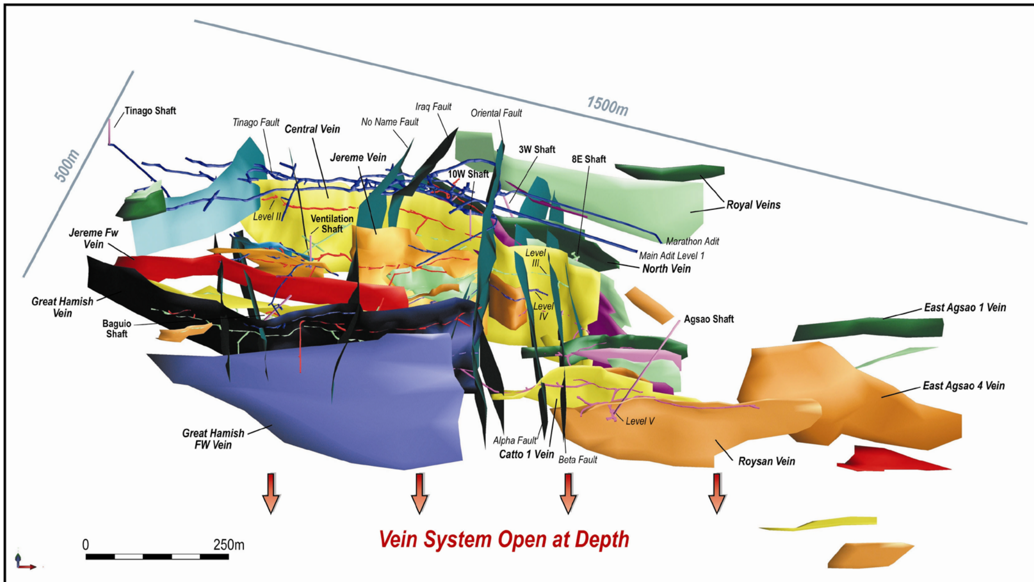
Figure 1. 3D model of the Co-O vein system and underground workings
