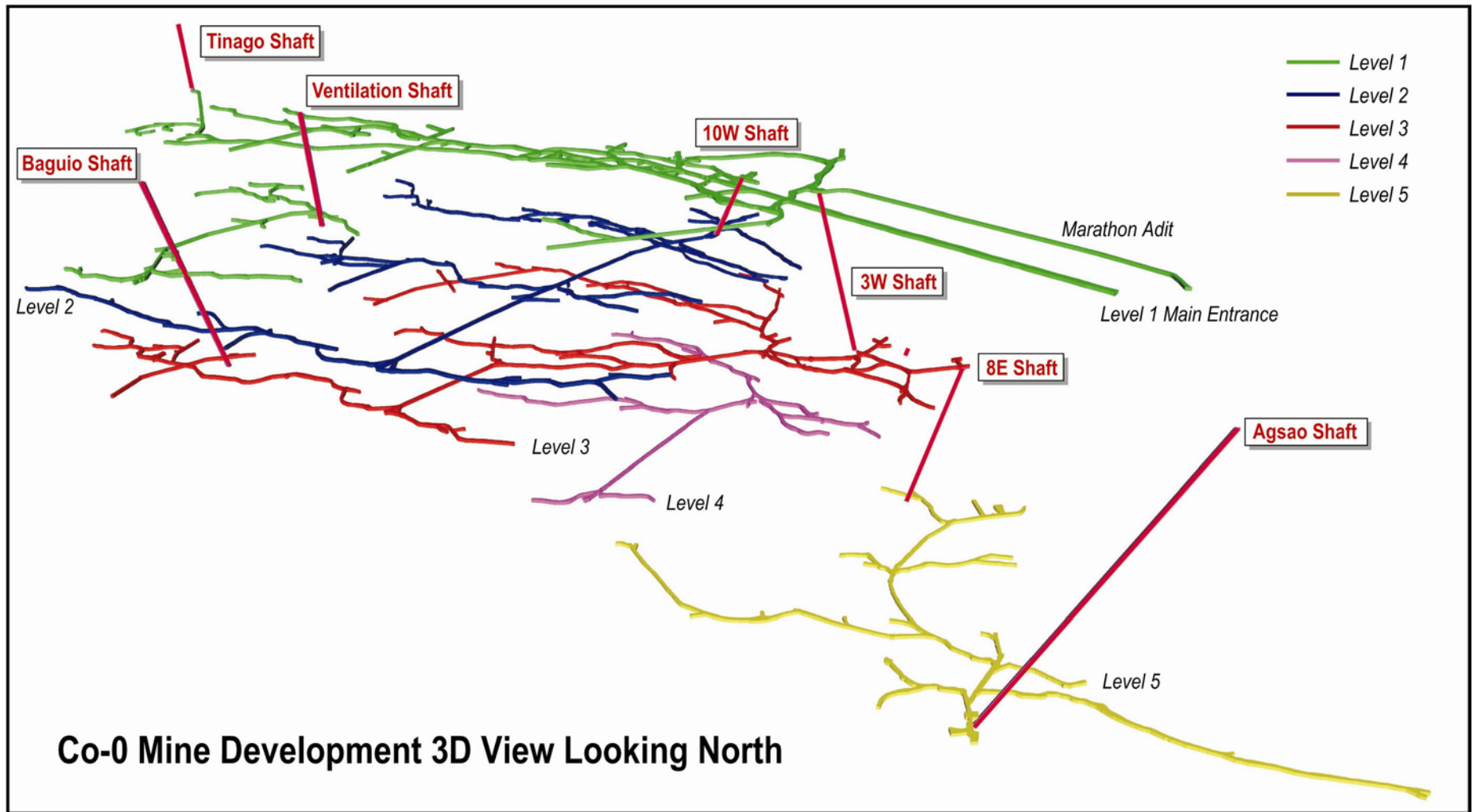
Figure 3. 3D view of the Co-O Mine underground workings.
