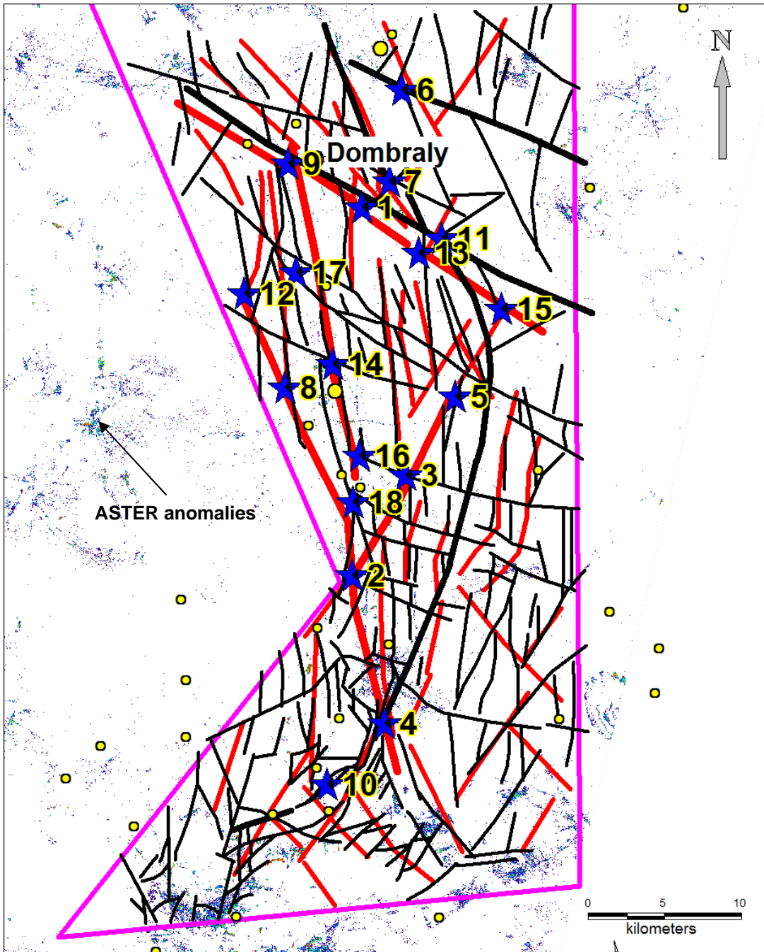
Figure 2 - Pilot Geophysical Survey Area with Primary Geophysical Target Positions and ASTER Anomalism
