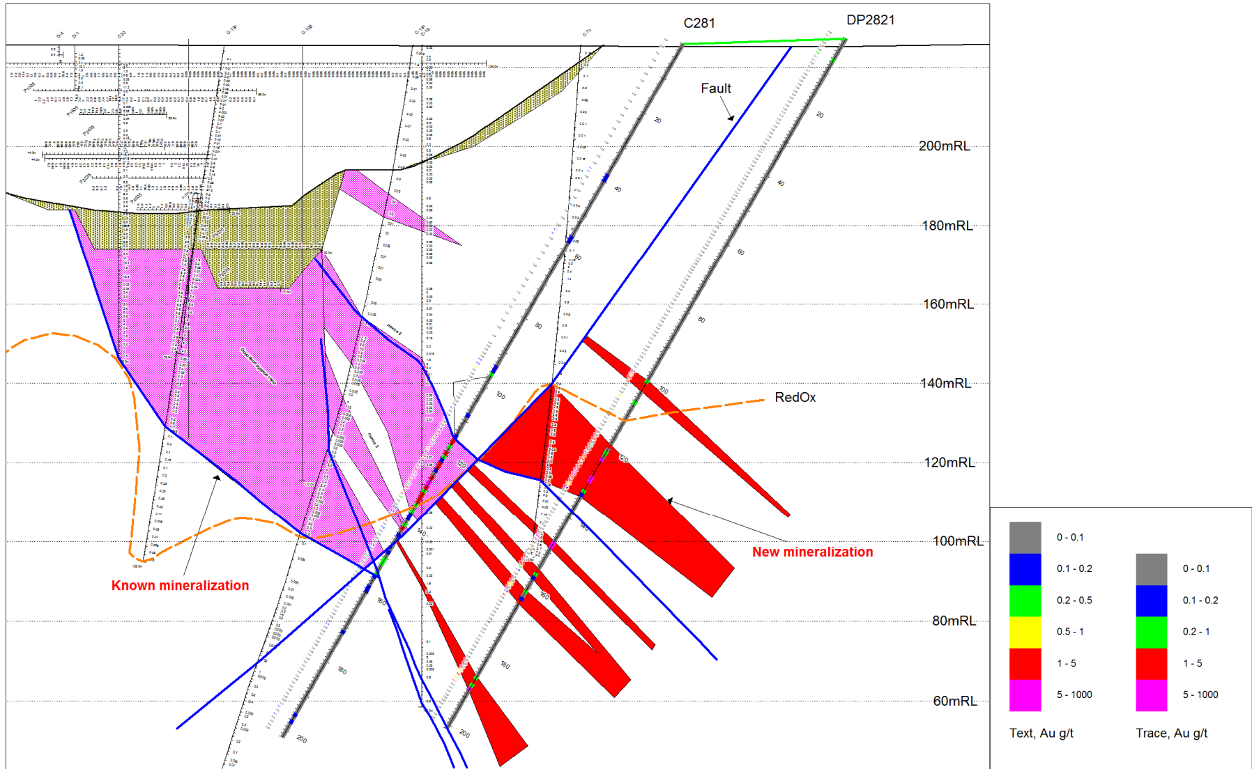
Figure 3 – Dombraly Cross Section along Line 28
