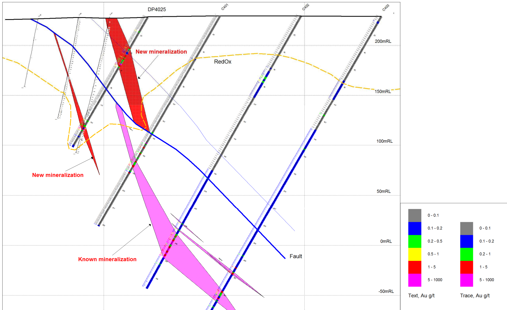
Figure 4 – Dombrały Cross Section along Line 40
