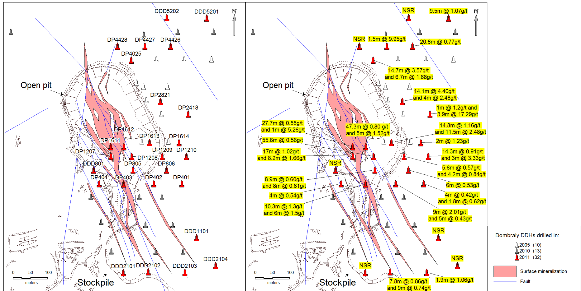
Figure 2 – Dombraly 2011 Diamond Drill Hole Positions and Major Intercepts
