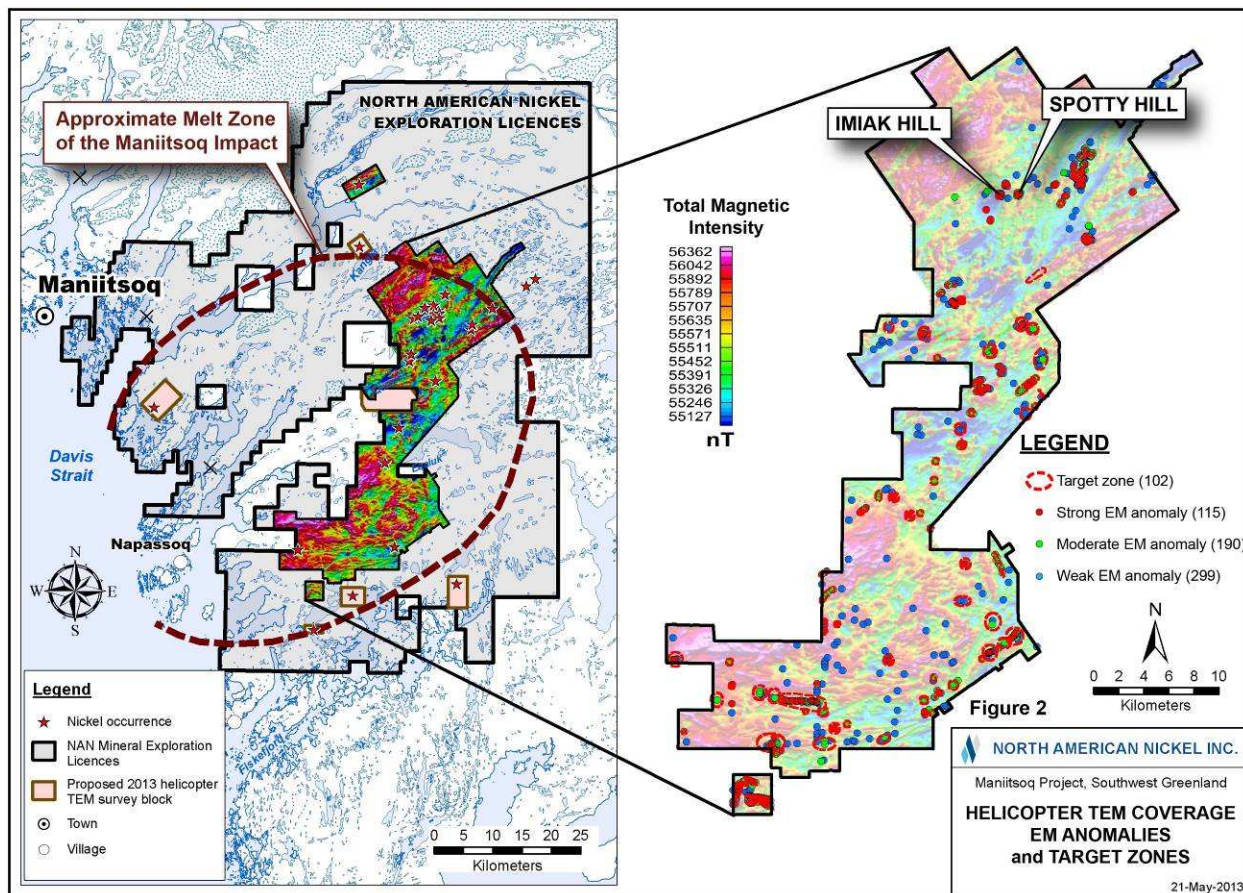
Figure 2: Plan map of the Maniitsoq project showing helicopter TEM coverage (area covered by colour magnetic images) and exploration target zones.
