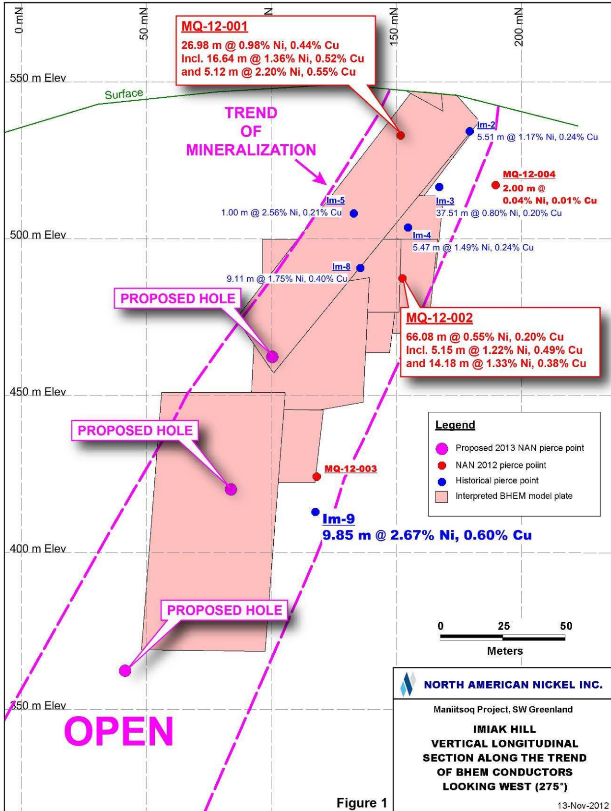
Figure 1: Longitudinal section (looking west) along the conductive trend associated with the Imiak Hill Mineralization showing approximate pierce points of proposed drill holes.
