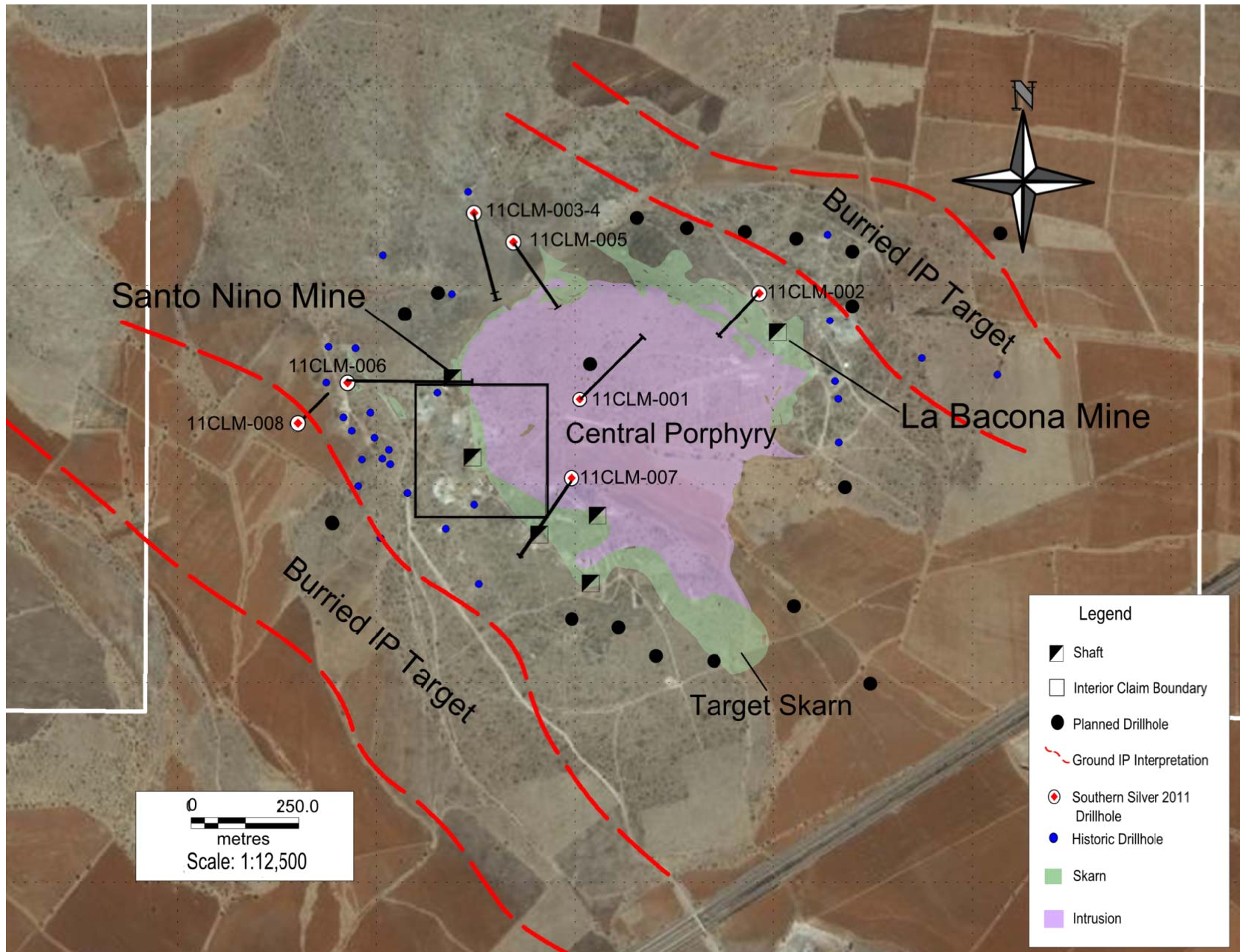
Figure 1: Plan view of the area of historic mining at the Cerro Las Minitas Project showing the distribution of current, historic and planned drill holes. Gravel covered geophysical targets, outlined in red, highlight the exploration potential of the project.
