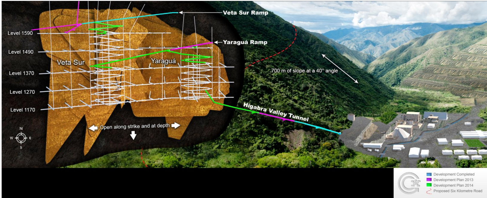
Figure 2 – Long Section of Development Plans and Proposed Infrastructure
