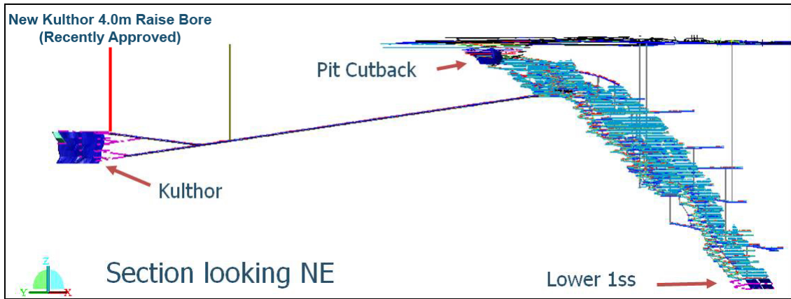
Figure 2B: Detail of planned Kulthor Development including new raise bore
