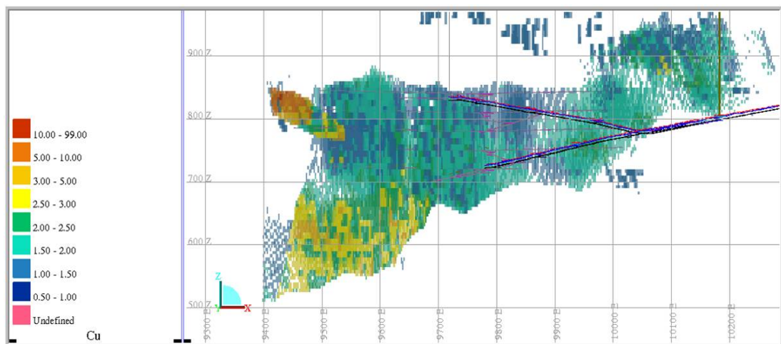
Figure 2C: Kulthor Copper Grade Blocks showing higher grade areas in south western end
