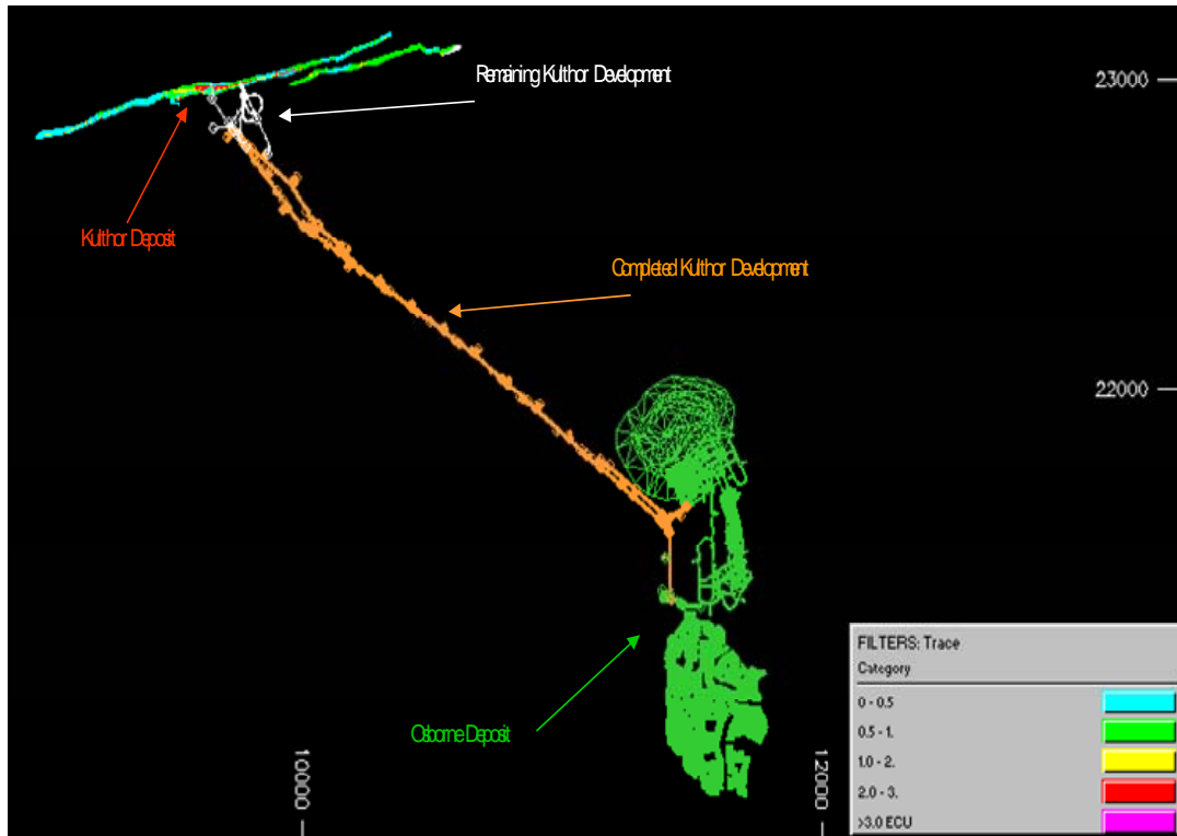
Figure 3: Plan view of Kulthor Underground Development showing 2.35 km completed decline. 150 metres remaining to access orebody
