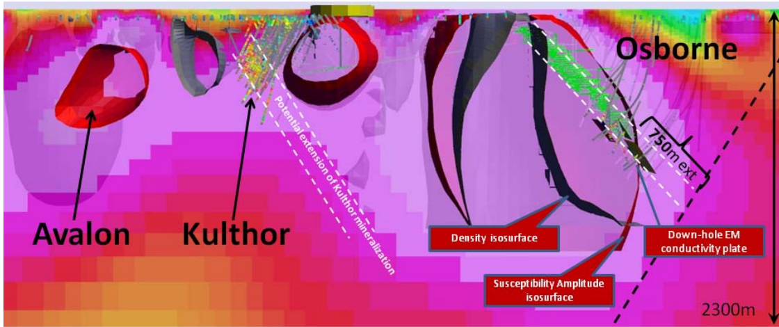
Figure 6: Potential depth extension for Osborne, Kulthor and Avalon Long Section (AB) through 3D VRMI inversion.
