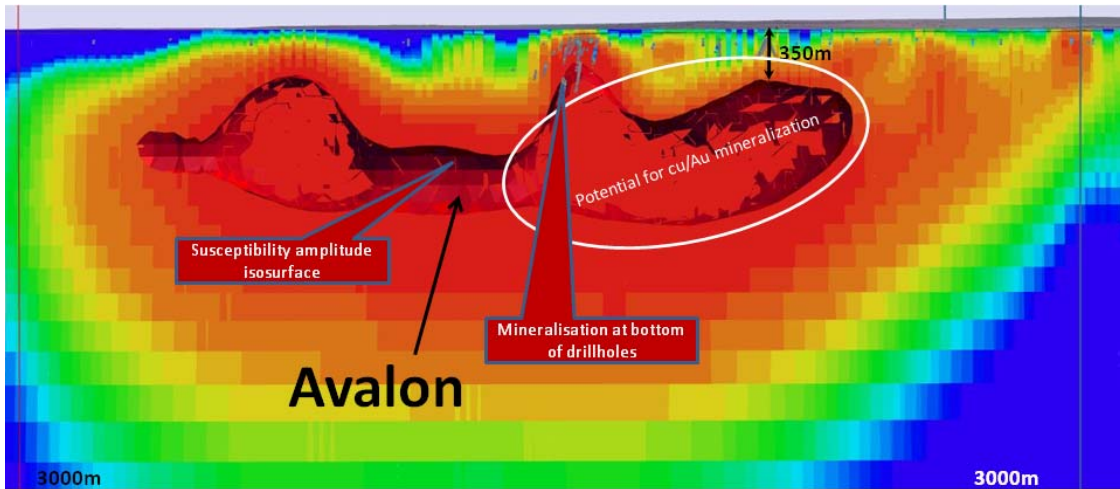
Figure 8: New Avalon anomaly (Long Section C-D axis from Figure 7)
