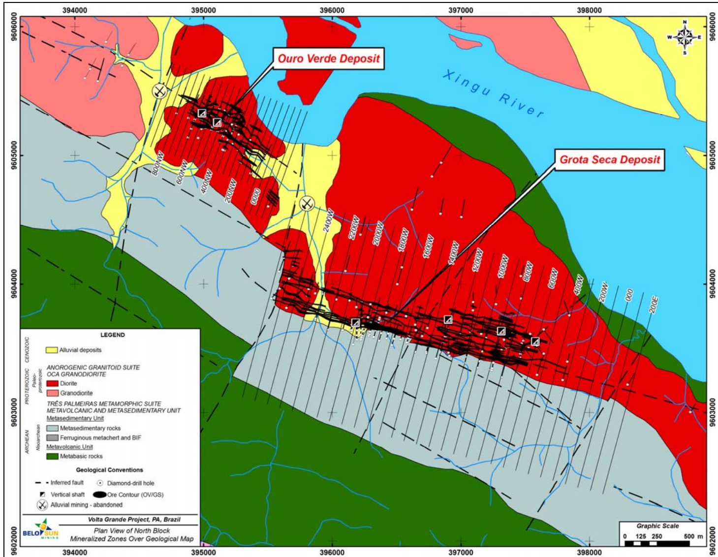
Figure 2 – Volta Grande Geological Map and Location of Ouro Verde and Grota Seca deposits
