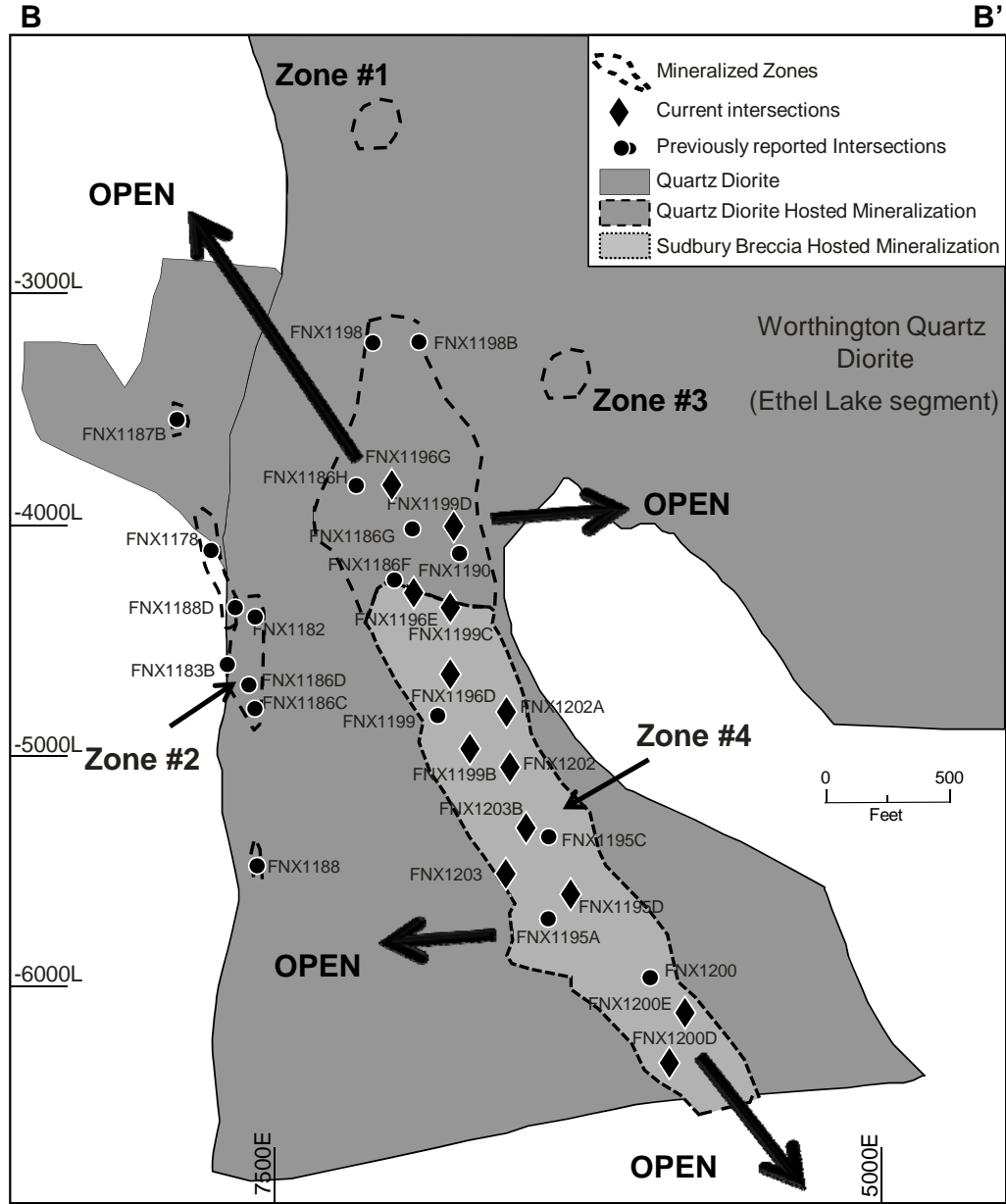
Figure 3: Long Section (Looking North – Grid A)
