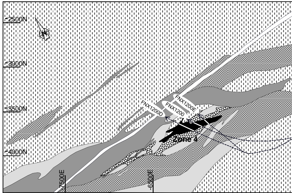
Figure 6: Level 6000 Mineralization
