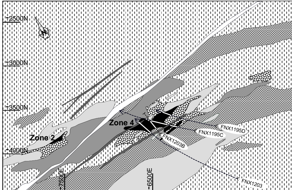
Figure 5: Level 5500 Mineralization
