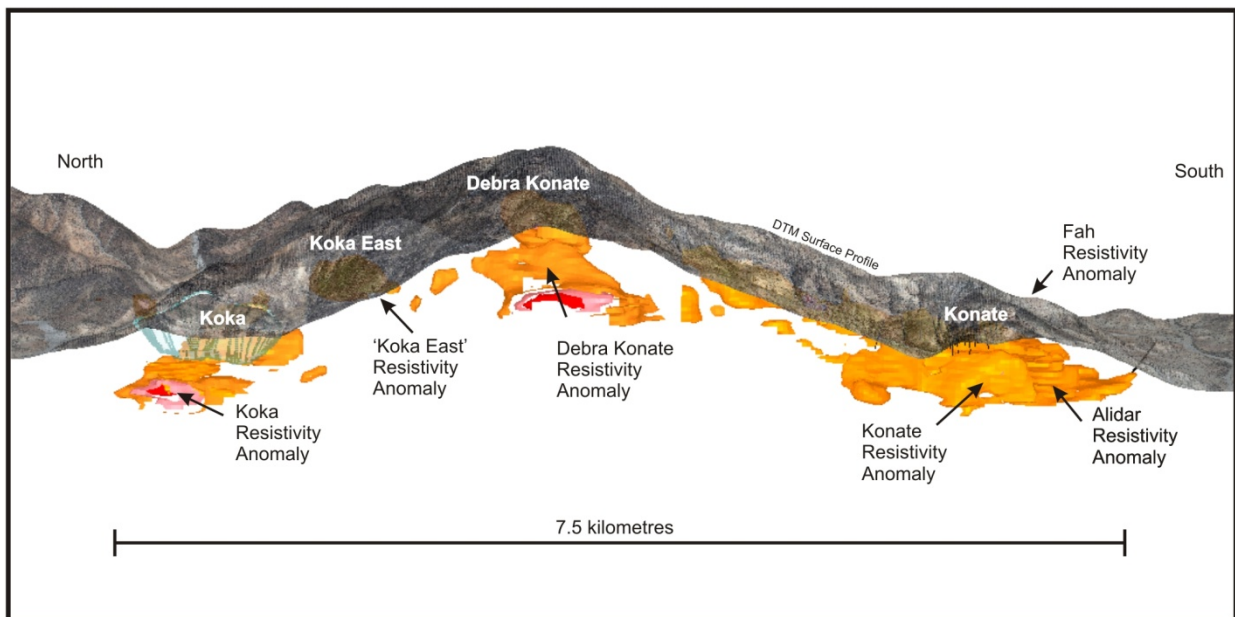
Long section – Koka-Konate corridor high priority IP resistivity anomaly drill targets
