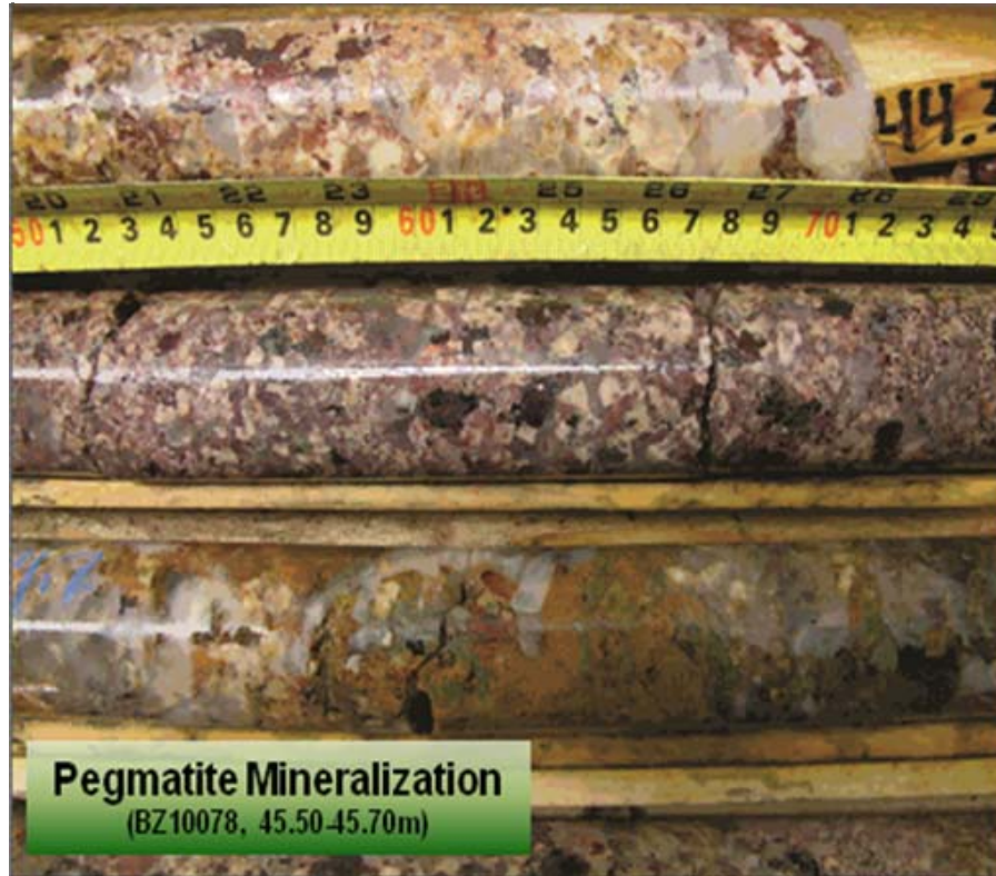
Figure 1. Drill Core Photos of Pegmatite and Granite, Strange Lake B-Zone Deposit, Québec
