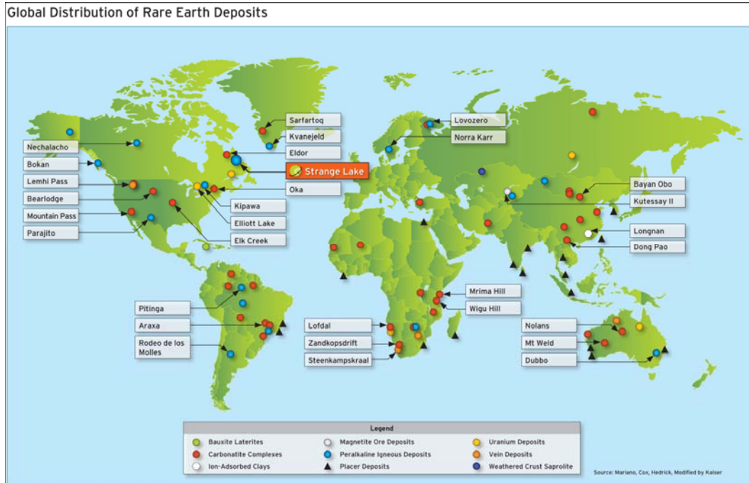
Figure 2 - Global Distribution of Rare Earth Element Deposits
