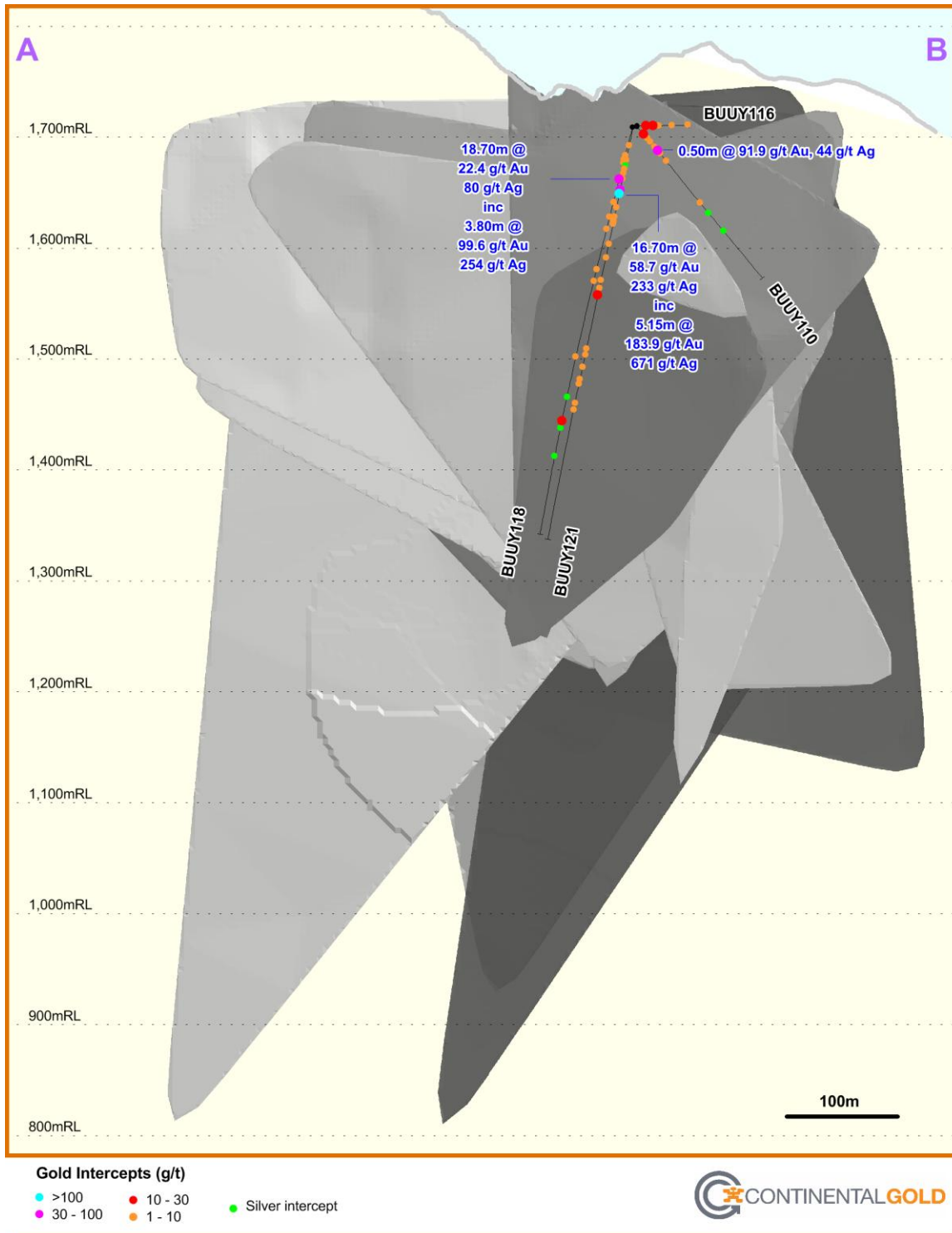
Figure 2 – Long Section, Veta Sur, showing new drilling highlights against the outlines of the October 2022 mineral resource envelope
