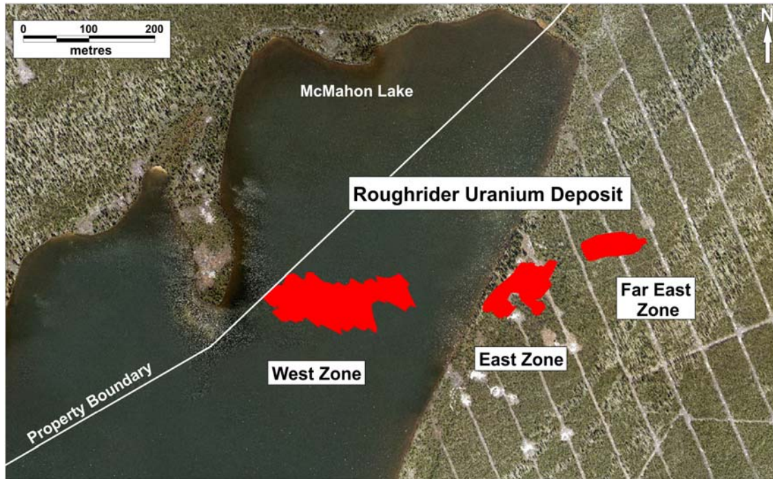
Figure 3. Aerial view of the Roughrider project. Outline of West zone is from Technical Report, January 15, 2011; outline of East Zone is from Technical Report, June 28, 2011; and outline of Far East Zone surrounds drill holes with anomalous radioactivity (news release dated September 6, 2011).
