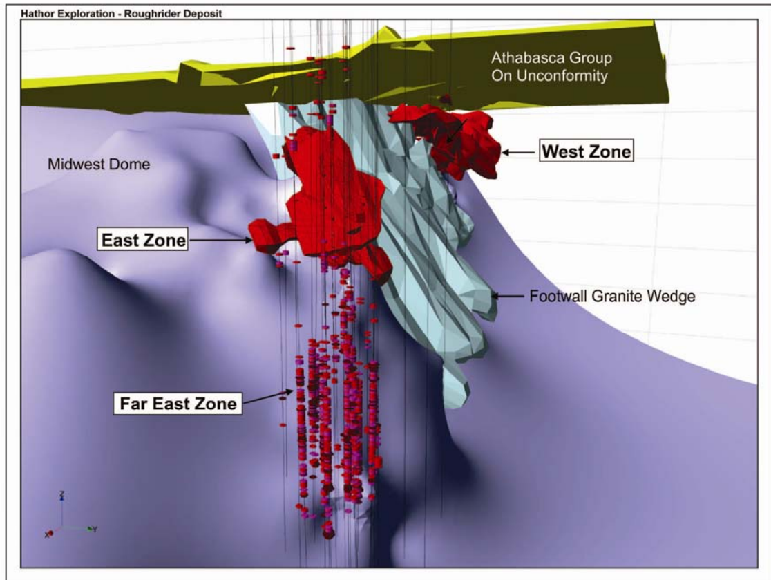
Figure 4. Three dimensional block model of the Roughridger Uranium Deposit, positioned mostly below the unconformity, on top of and peripheral to the Midwest Archean dome. Outline of West Zone is from Technical Report, January 15, 2011; outline of East Zone is from Technical Report, June 28, 2011; and purple outline of Far East Zone surrounds drill holes with anomalous radioactivity (news release dated September 6, 2011).
