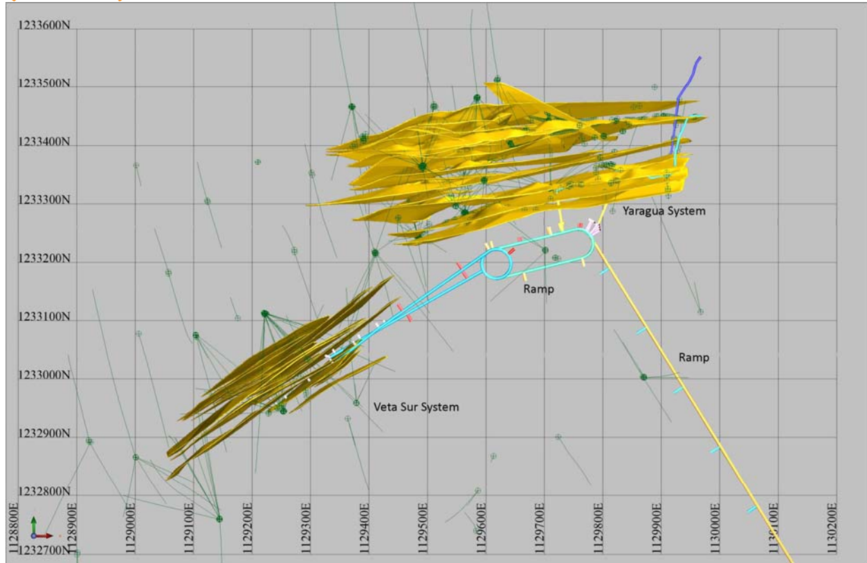
Figure 2: 3D Model of Yaragua and Veta Sur Systems with Proposed Developments (Plan View)
