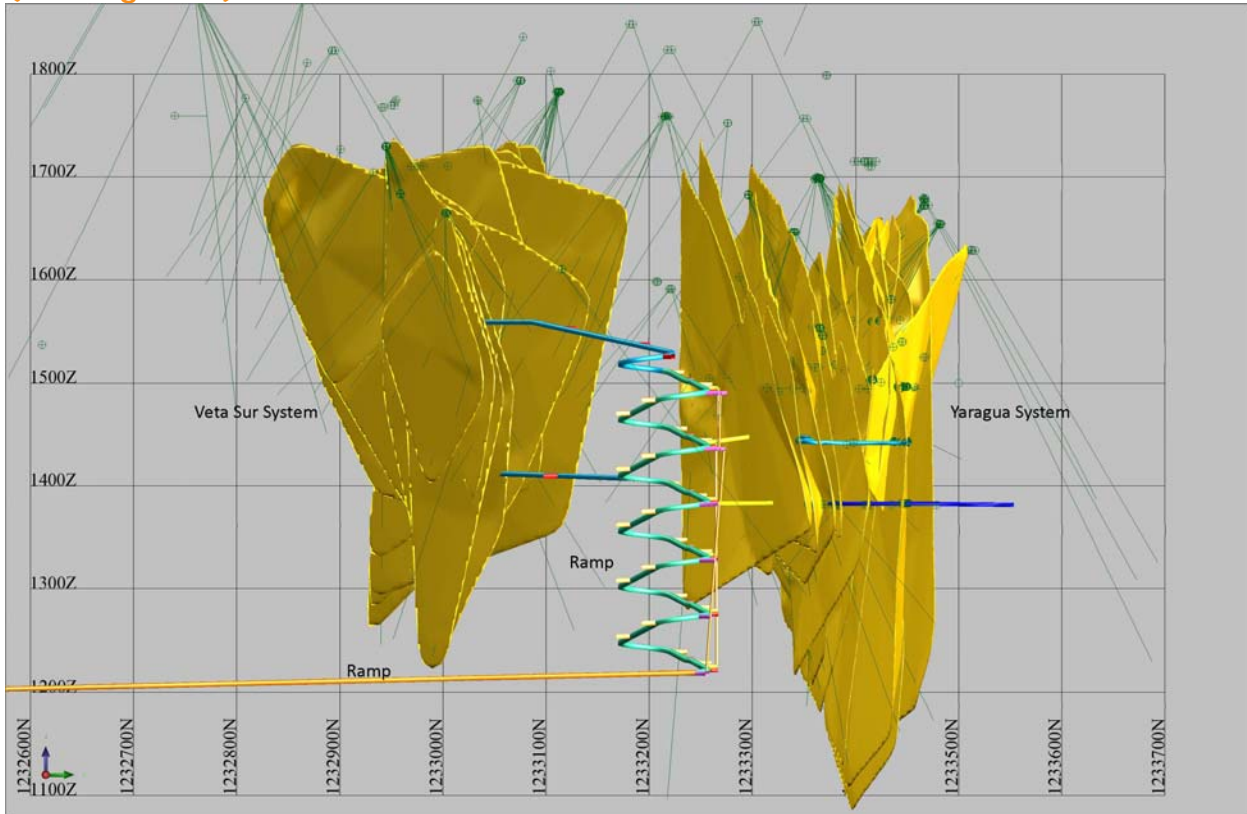
Figure 3: 3D Model of Yaragua and Veta Sur Systems with Proposed Developments (Looking West)
