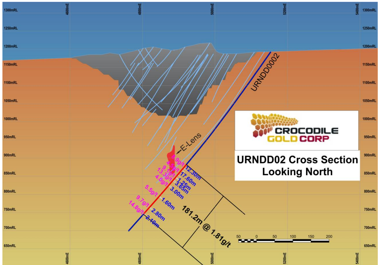
Figure 6: URNDD02 Cross Section
