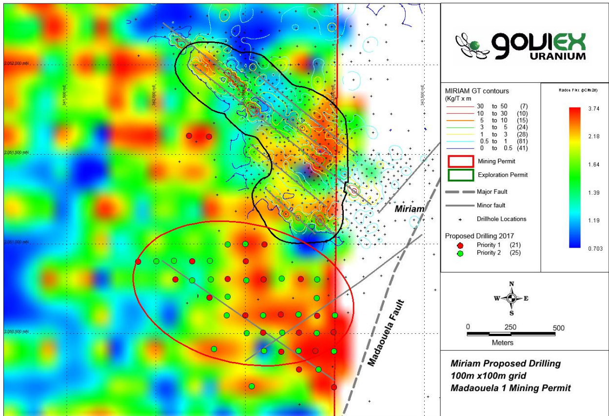
Figure 3. Miriam planned open-pit outline, radon anomaly and planned delineation drilling
