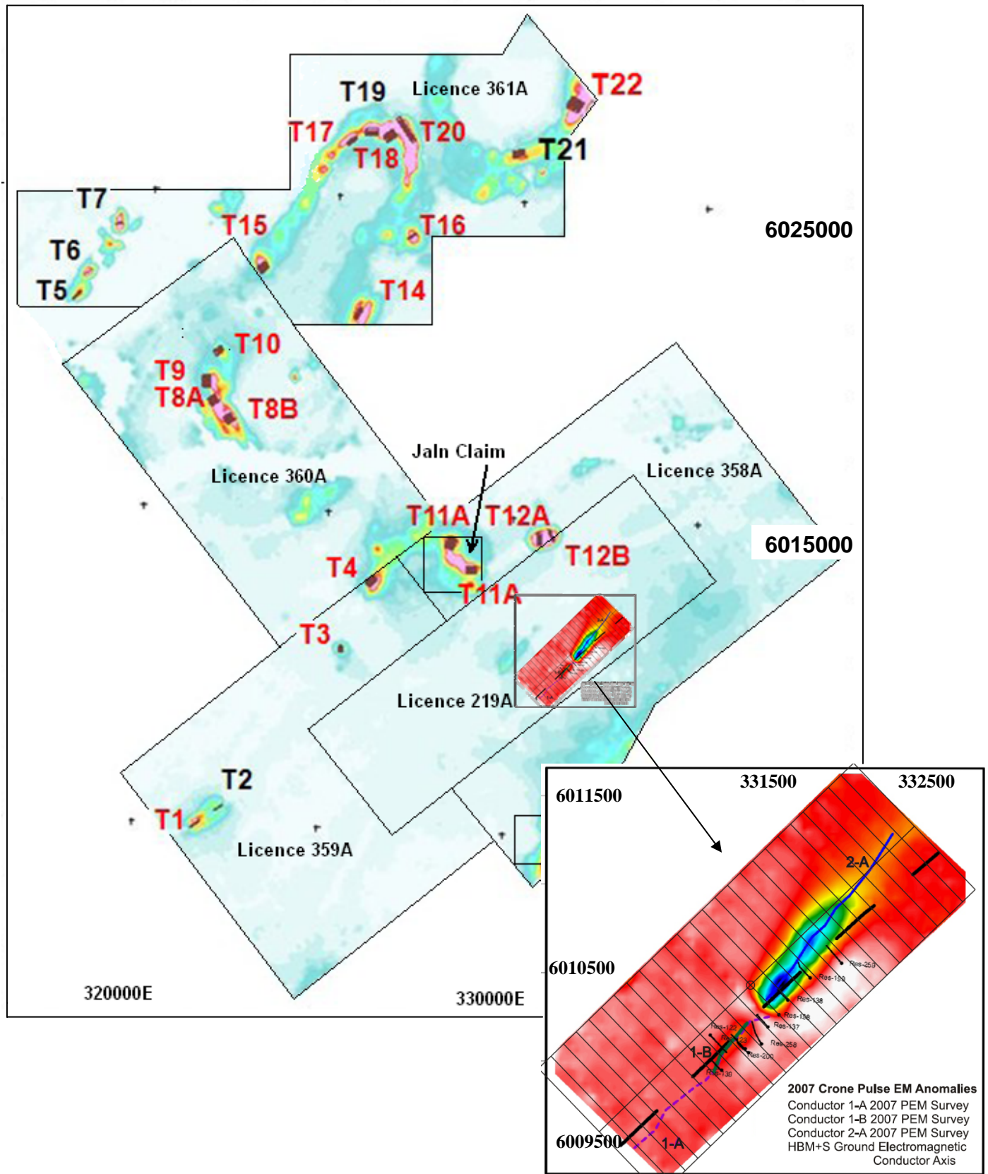
Geotech VTEM Time Domain EM Drill Hole Targets and Inset showing Crone Geophysics Pulse EM Survey conductor anomalies.
