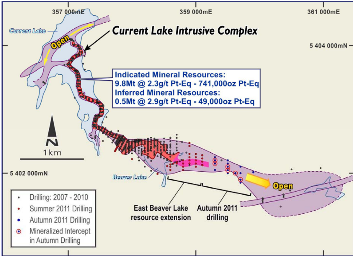
Figure 1. Current Lake Intrusive Complex showing the mineral resource extension at East Beaver Lake in purple.
