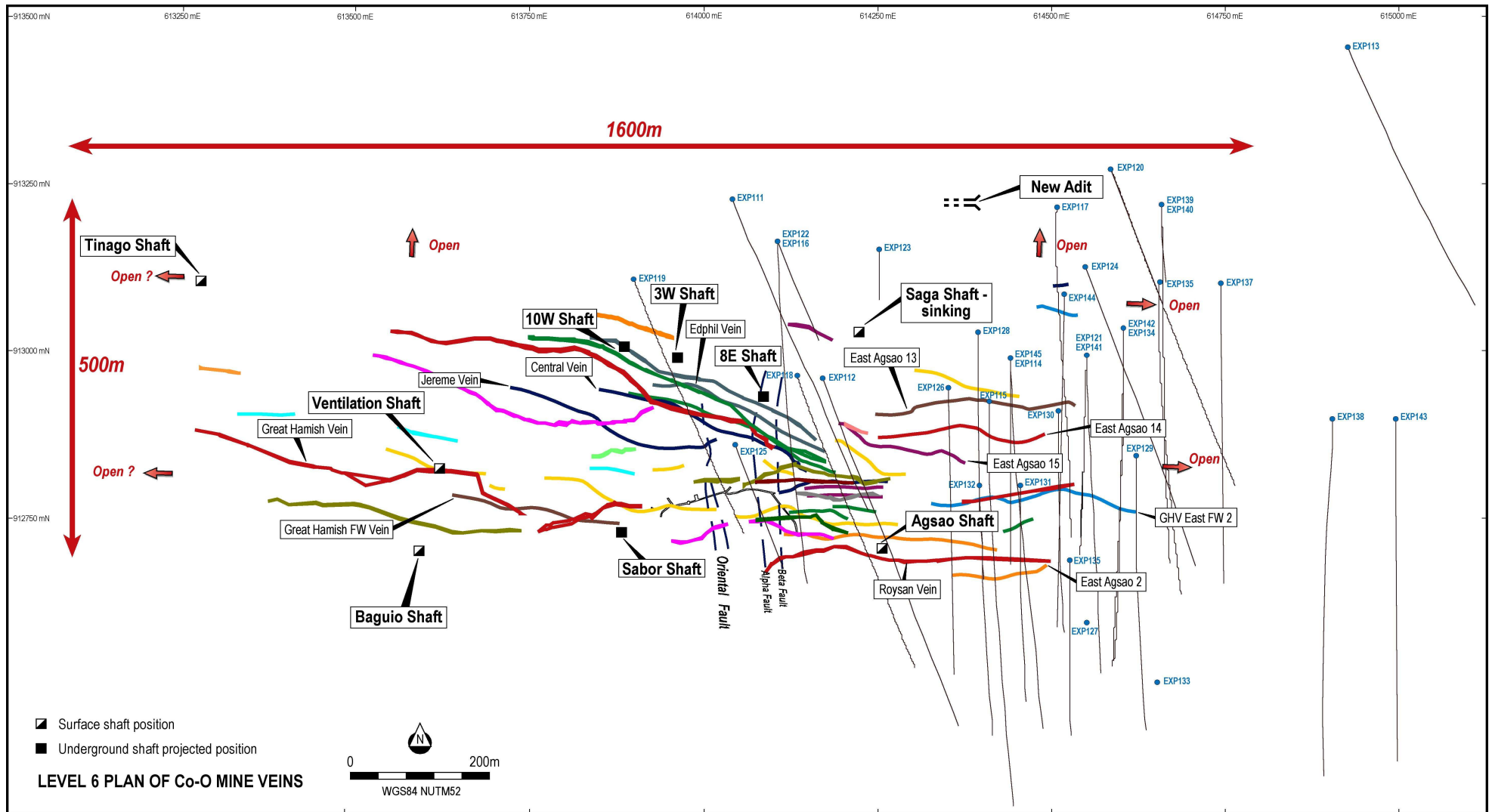
Figure1. Map of the Co-O Mine Level 6 plan showing the locations of new drill holes EXP111 to EXP145.
