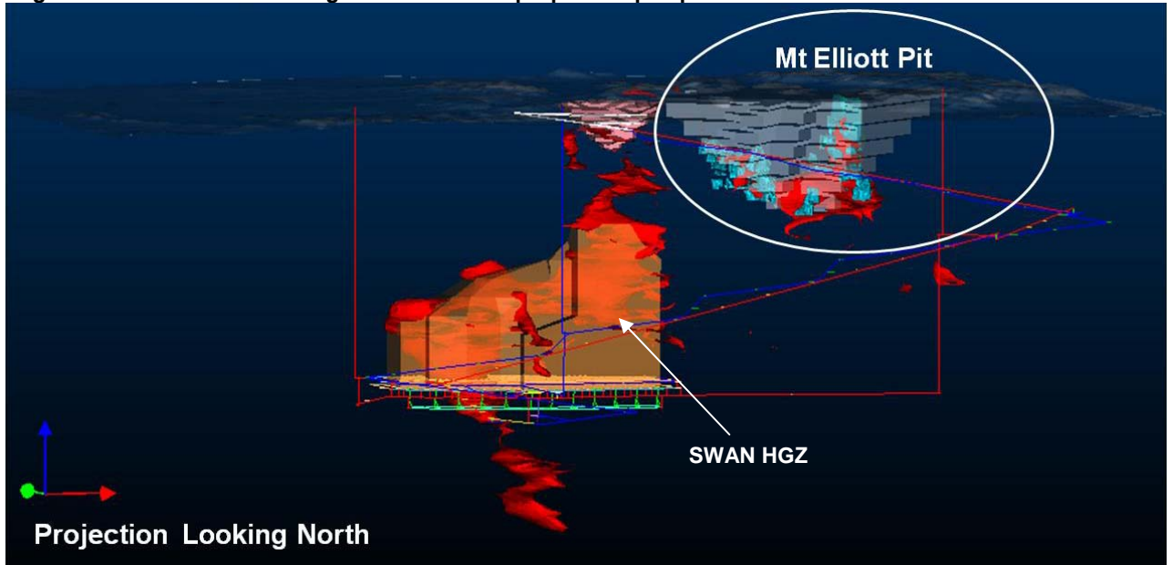
Figure 1: Mount Elliott showing SWAN HGZ and proposed open pit
