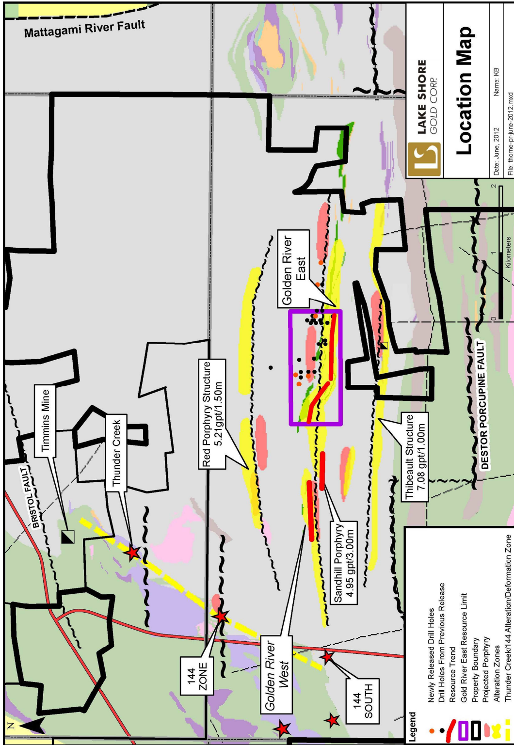
Figure 1. Plan View
